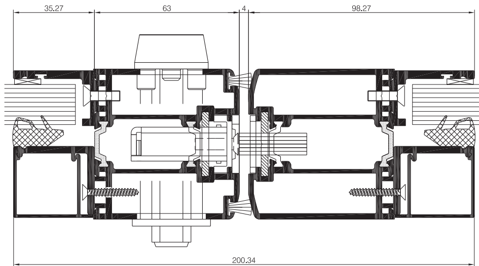
General Arrangement showing Comar 7P.i CD Double Door Meeting Stiles
