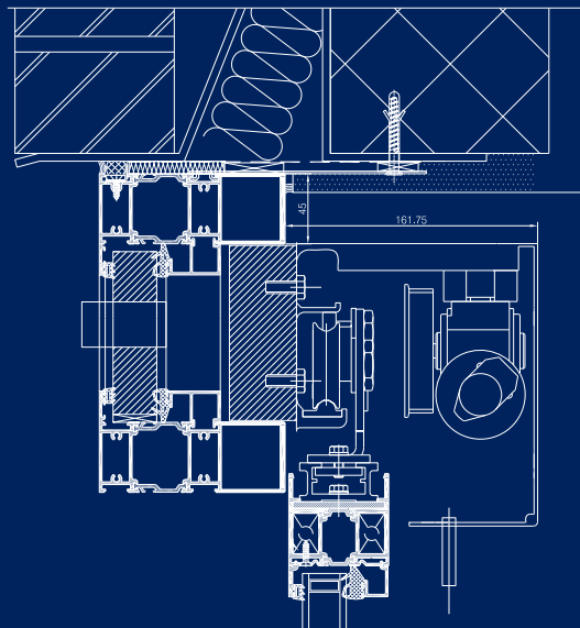
General Arrangement showing Comar 7P.i CD Automatic Door Head Detail
