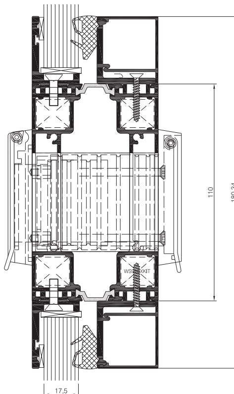
General Arrangement showing Comar 7P.i CD Security Midrail Option with Axim letterplate
