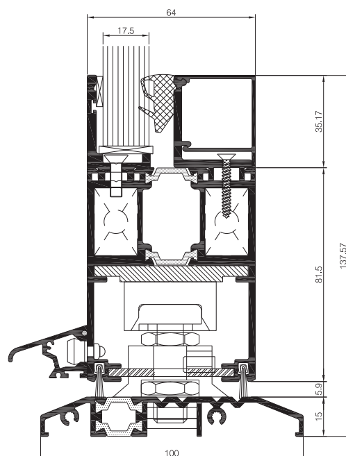
General Arrangement showing Comar 7P.i CD with a low-rise thermally broken sill option
